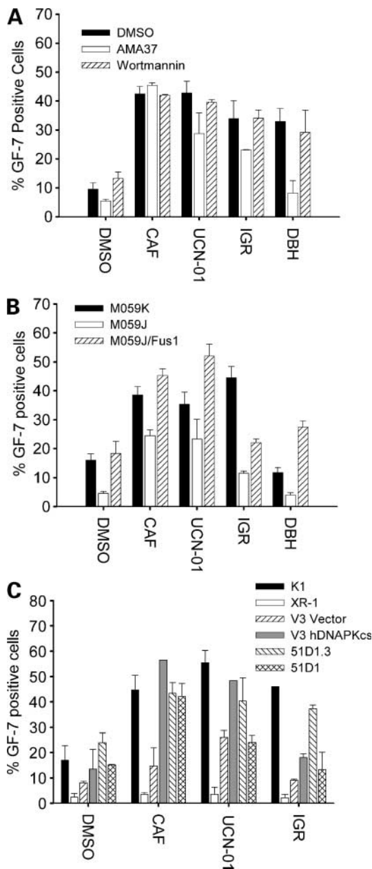
Figure 1. Effect of G_2 checkpoint inhibitors on cells lacking DNA-PK or NHEJ activity. A , MCF-7 mp53 cells were exposed to DMSO, 20 \mu mol/L AMA37, or 200 nmol/L wortmannin 30 min before irradiation with 6.5 Gy. Sixteen hours later, when arrested in G_2 , cells were exposed to checkpoint inhibitors plus nocodazole for 8 h and harvested as described in Materials and Methods. GF-7-positive cells represent those trapped in mitosis. B , MO59 cells were irradiated and treated as in A . C , CHO cells were irradiated with 6.5 Gy. Eight hours after ionizing radiation, checkpoint inhibitors and nocodazole were added for 4 h. Columns, average between different experiments ( n \geq 2 ); bars, SD.
