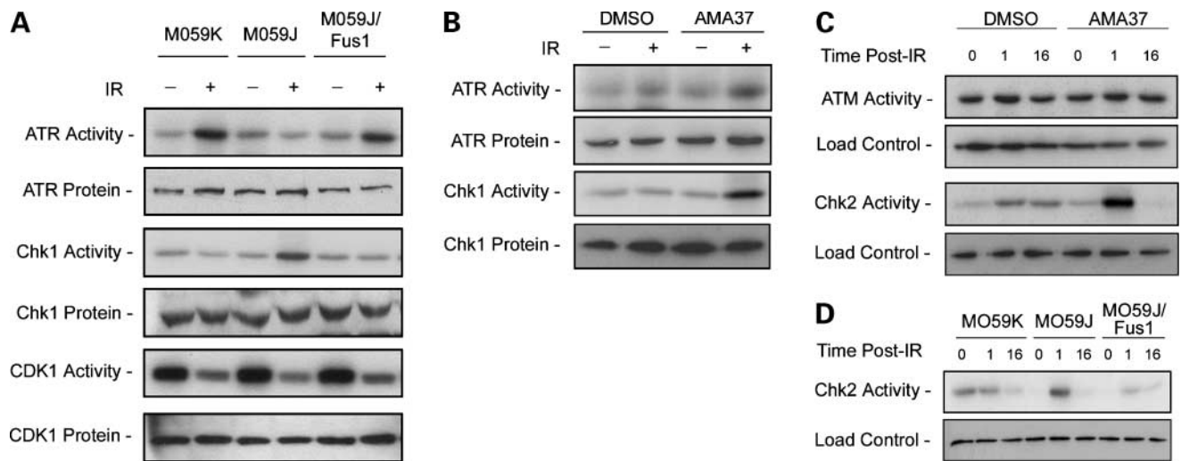
Figure 3. Overactivation of Chk1 and Chk2 in DNA-PK-deficient cells. A , ATR, Chk1, and CDK1 activity in irradiated cells. Cells were harvested 16 h after mock irradiation (–) or exposure to 6.5 Gy (+). Cellular levels of ATR, Chk1, and CDK1 protein were measured by Western blotting, and their kinase activity was measured in immunoprecipitates as described in Materials and Methods. B , MCF-7 mp53 cells were treated without or with AMA37 30 min before irradiation, and cellular levels and kinase activity of ATR and Chk1 were measured as above 16 h after irradiation. C , ATM and Chk2 activity in irradiated MCF-7 mp53 cells harvested 1 or 16 h after ionizing radiation (IR). D , Chk2 kinase activity of M059 cells measured at 1 or 16 h after ionizing radiation.
