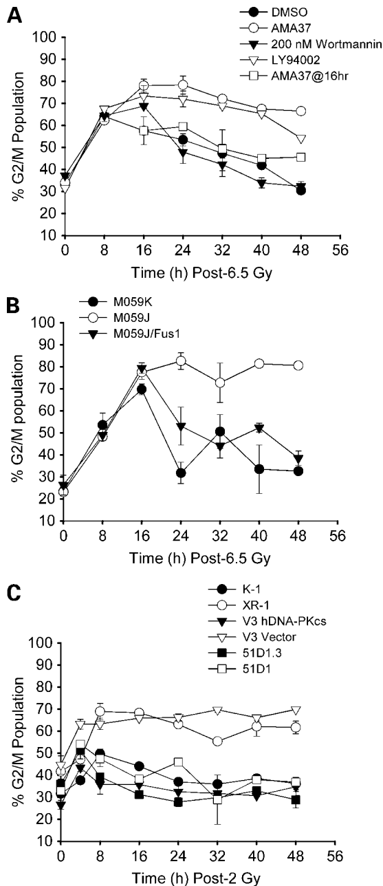
Figure 2. Effect of ionizing radiation on G_2 arrest in cells lacking DNA-PK or NHEJ activity. Cells were irradiated at time 0 and sampled at the indicated times, and the G_2 -M populations were quantitated using flow cytometry. A , MCF-7 mp53 cells were exposed to DMSO, 20 \mu mol/L AMA37, 200 nmol/L wortmannin, or 50 \mu mol/L LY294002 30 min before irradiation with 6.5 Gy. Another cell population was irradiated with 6.5 Gy, and AMA37 was added 16 h later. Cells were harvested at the indicated times and analyzed by flow cytometry. B , MO59K, MO59J, or MO59J/Fus1 cells were exposed to 6.5 Gy. C , CHO cells were exposed to 2 Gy. Points, average between different experiments ( n \geq 3 ); bars, SD.
