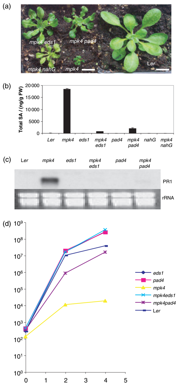
Figure 4. Mutations in EDS1 and PAD4 suppress SA-dependent defense activation in mpk4 .
