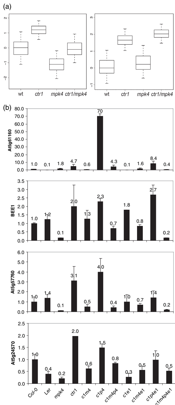
Figure 7. mRNA accumulation patterns in WT and mutants determined by transcriptomics and real-time quantitative PCR.
