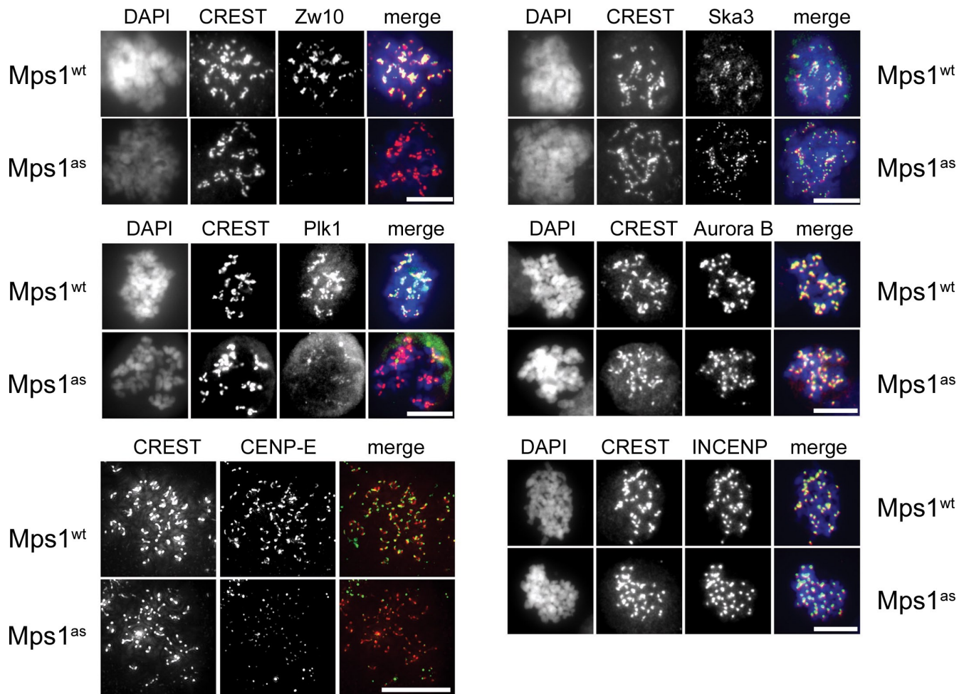
Figure S2. Mps1 kinase activity is continuously required to maintain SAC effectors at kinetochores. Cells treated as in Fig. 7 were stained with antibodies to the indicated SAC/kinetochore proteins (green), CREST antiserum (red), and DAPI (blue). All images were acquired via widefield microscopy except for CENP-E, which was acquired and deconvolved on an image restoration microscope (Deltavision). Bars, 10 \mu m.
