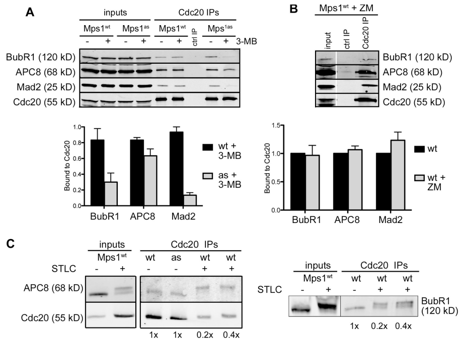
Figure 3. Mps1 directs the assembly of Cdc20 inhibitory complexes in interphase. (A) Mps1 wt and Mps1 as cells were treated with 3MB-PP1 for 2 h. Extracts were immunoprecipitated with antibodies to Cdc20 and resolved by SDS-PAGE. Levels of BubR1, APC8, Mad2, and Cdc20 in each IP were determined by quantitative immunoblotting. The ratio of each protein to Cdc20 was computed and normalized to ratios obtained from untreated Mps1 wt cells (= 1.0). (B) Mps1 wt cells were treated with ZM for 2 h and processed as in A. White line indicates that intervening lanes have been spliced out. (C) Interphase and mitotic Cdc20 IPs were electrophoresed on 6% gels to resolve mitotically phosphorylated APC8 (left) and BubR1 (right) polypeptides as distinct species. Numbers at the bottom are loading amounts. Black lines indicate that intervening lanes have been spliced out. ctrl, control. Error bars indicate SEM.
