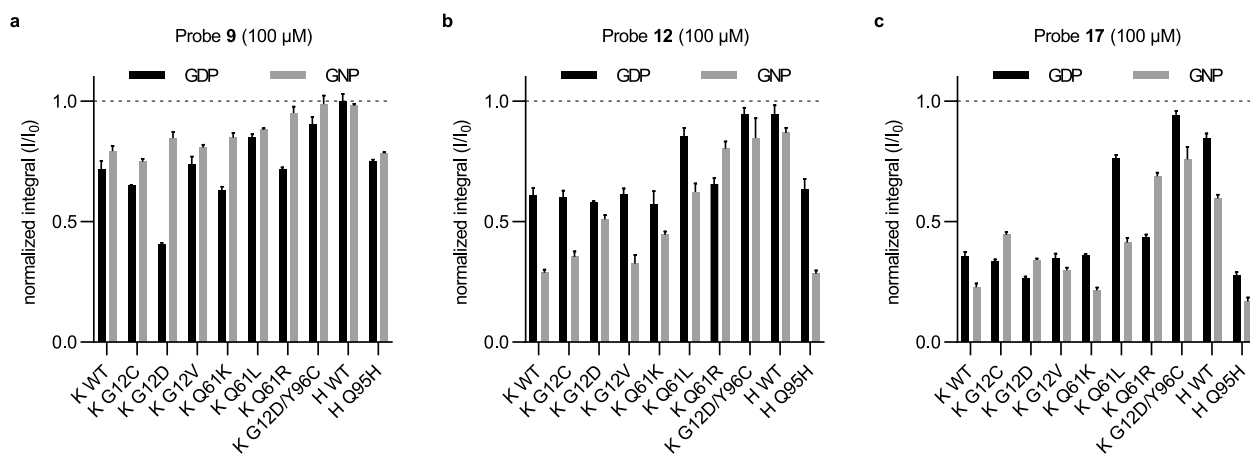
Figure 3. ^{19}\text{F} CPMG NMR spectroscopy detects a variety of oncogenic KRas proteins. Normalized integrals ( I/I_0 ) from ^{19}\text{F} CPMG NMR spectra (160 ms) of 100 \mu\text{M} 9 (a), 12 (b), or 17 (c) in the presence of 6 \mu\text{M} KRas or HRas proteins; values are means \pm errors propagated from the SDs of I and I_0 ( n = 3 ).
