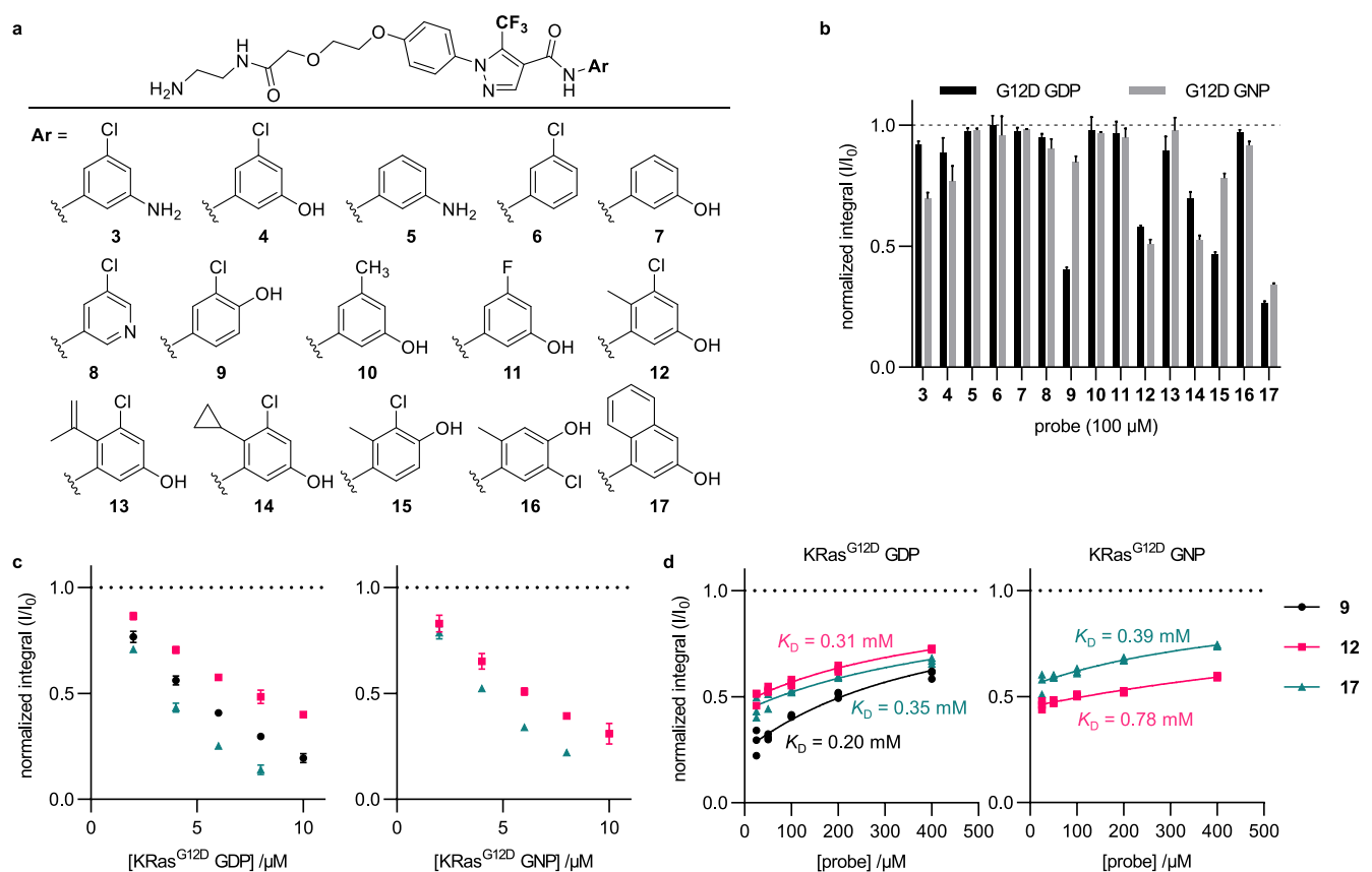
Figure 2. SAR of SIIG binders enables more sensitive detection of KRas G12D . (a) Chemical structures of SIIG binders. (b) Normalized integrals ( I/I_0 ) from ^{19}\text{F} CPMG NMR spectra (160 ms) of probes (100 \mu\text{M} ) with KRas G12D (6 \mu\text{M} ); values are means \pm errors propagated from SD ( n = 3 ). (c) Effect of varying KRas G12D concentration on I/I_0 ; values are means \pm errors propagated from SD ( n = 3 ). (d) Effect of varying probe concentration on I/I_0 ; [\text{P}]_0 = 6 \mu\text{M} for probes 9 and 12, 3 \mu\text{M} for probe 17; individual points shown ( n = 3 ); data fit to eq 1 (SI).
